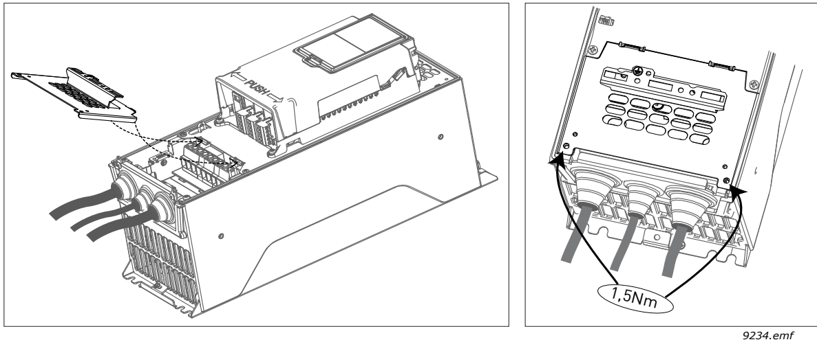
Figure 34. Re-mounting of cover components
