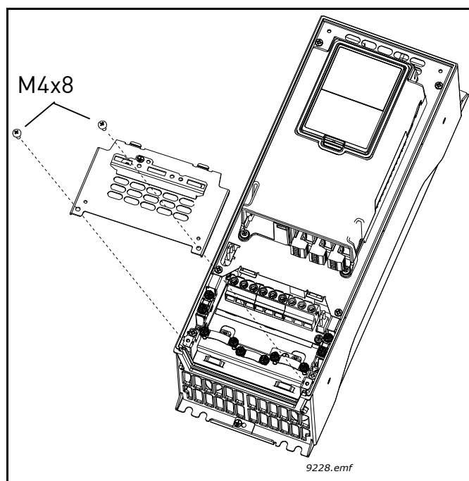
Figure 27. Removing screws
